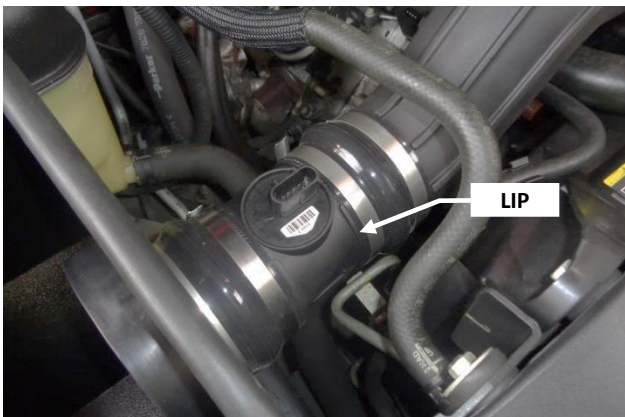
26. Push coupling (14) up against the lip on the MAF sensor and tighten the sensor clamp. (Do not yet tighten the tube clamp.)
