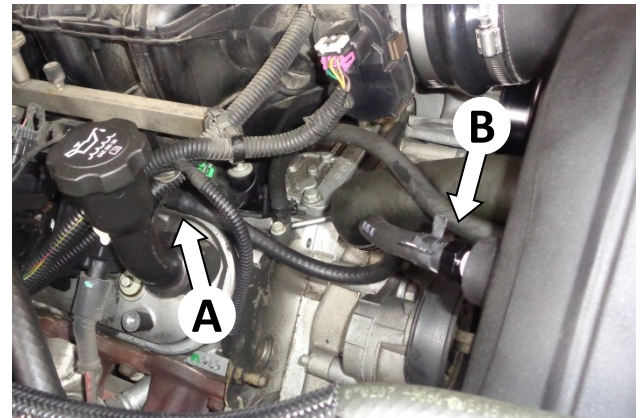
28. Push one end of hose (11) onto engine PCV tube (A). Cut the hose to length and secure it to the barbed fitting (B) with the pinch clamp (10).
