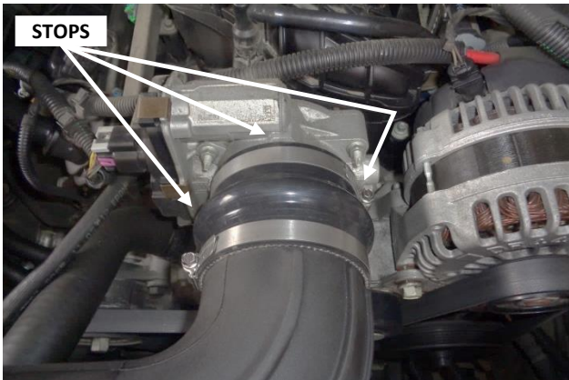
25. Push coupling (12) up against the stops on the throttle body opening and tighten the throttle body clamp. (Do not yet tighten the tube clamp.)
