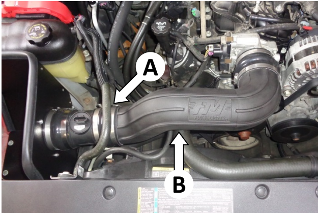
24. Install the intake tube in the vehicle. The tube will pass under the coolant overflow line (A), and over the two radiator lines (B).
