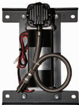
Air Accessory Mounting Kit 2497 shown with 9287 compressor
