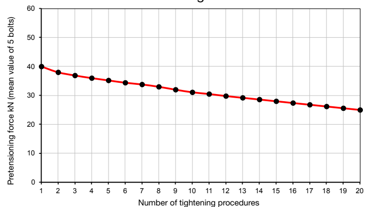
Pretensioning force curve
