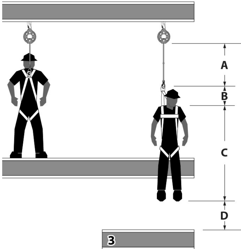
Figure 3 - Minimum Clear Fall Requirement: ANSI Class A Self Retracting Lanyard
