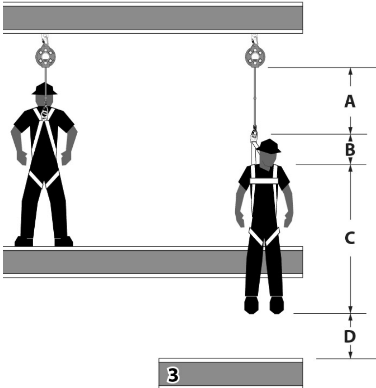
Figure 4 - Minimum Clear Fall Requirement: ANSI Class B Self Retracting Lanyard
