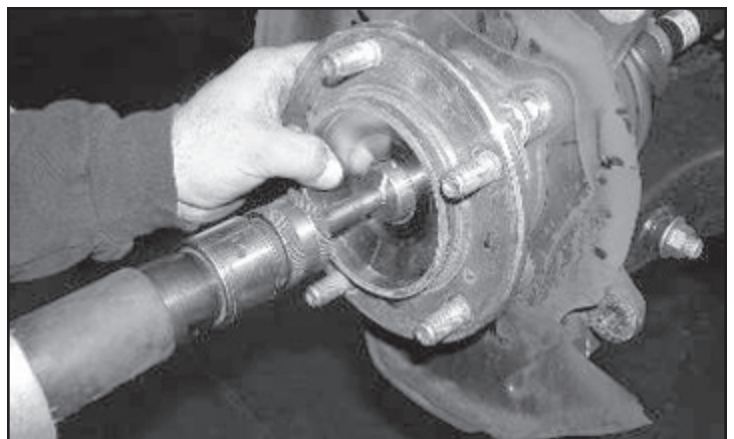
FIGURE 19 - STEP 7
