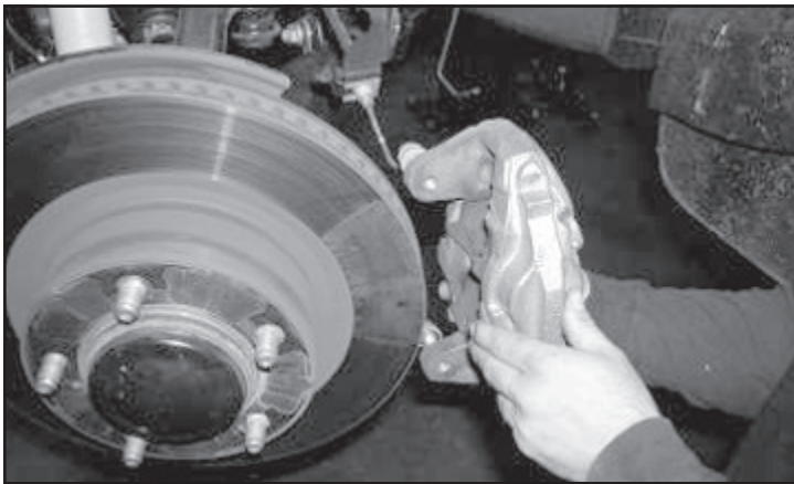
FIGURE 15 - STEP 7
