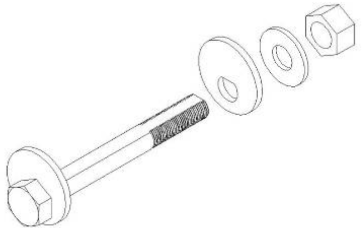
Assembly of the FT292 Alignment Cam
