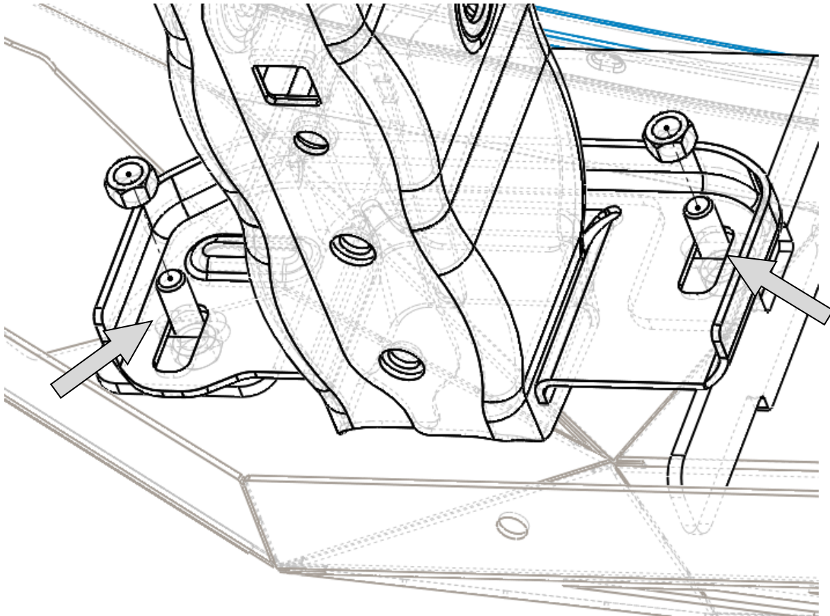
Figure 5 – FRAME FASTENER INSTALLATION LOCATION
