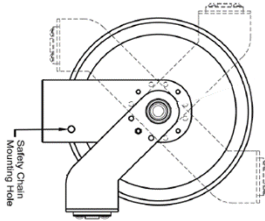
Figure 2-5 EVOREEL Cable Guide Bracket Adjustment
