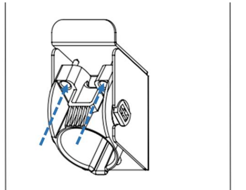
Figure 2-22 Lock screws
