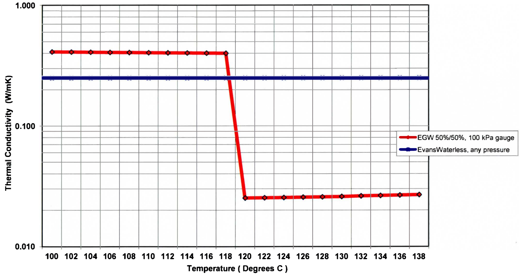
Figure 2 Thermal Conductivity of the Liquid and Vapor Phases of Water-Based Coolant vs. Evans Waterless (The vapor phase of water-based coolant has almost no thermal conductivity.)
