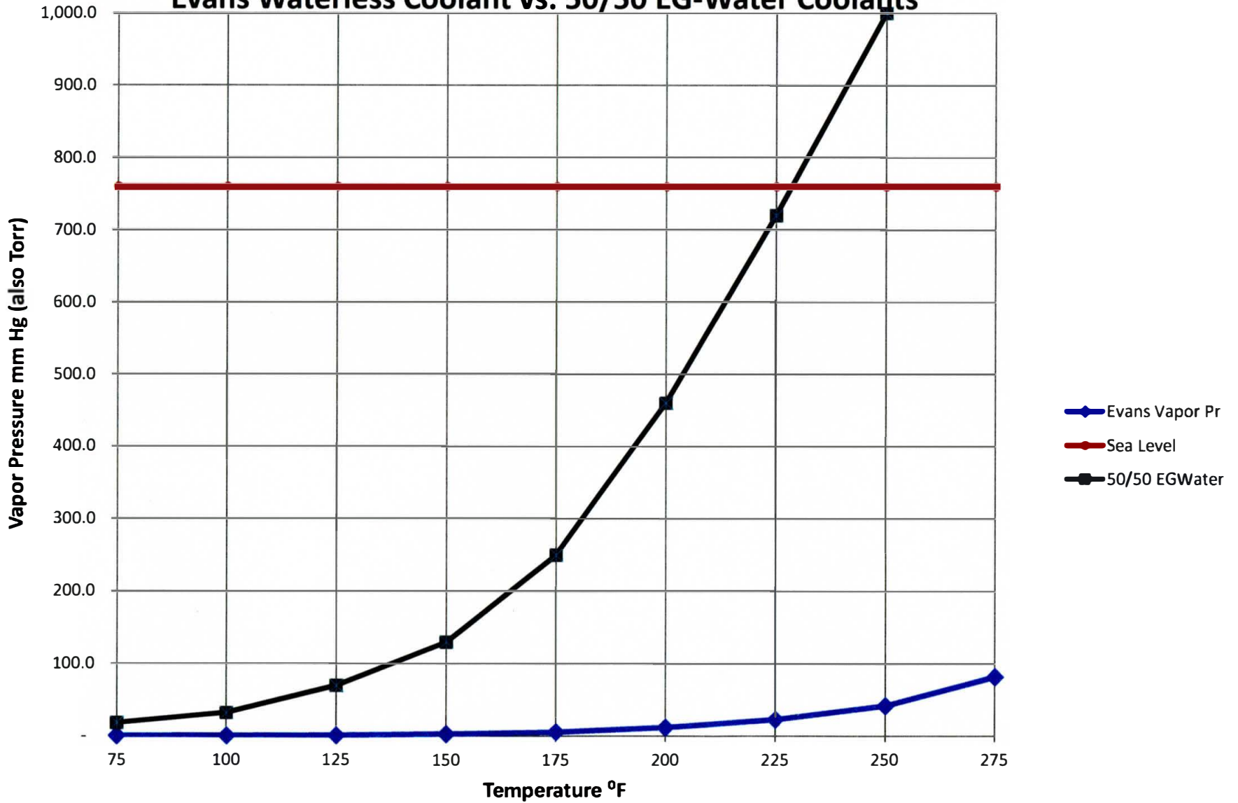
Figure 1 Comparison of Vapor Pressures Evans Waterless Coolant vs. 50/50 EG-Water Coolants
