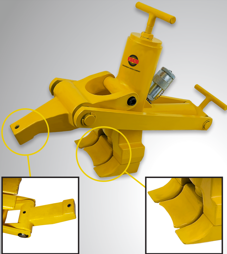
Redesigned replaceable clamping jaw.
