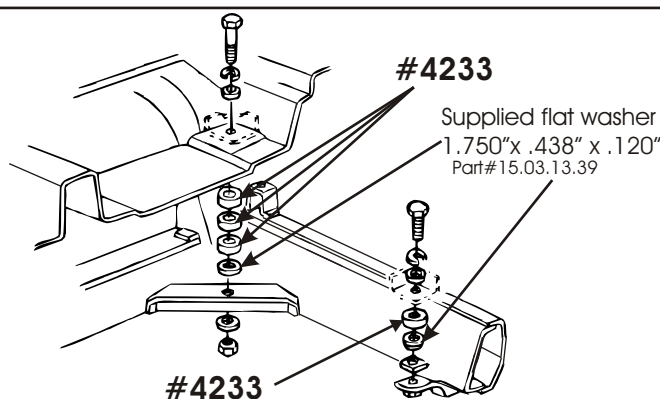
Set # 3.4153 63-64 Seat belt mount cushion positions. Only the cushions and washers are supplied, customer must reuse all O.E. hardware.
