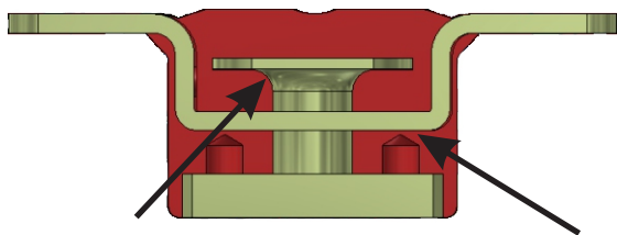
Side view (cutaway) showing safety interlock
