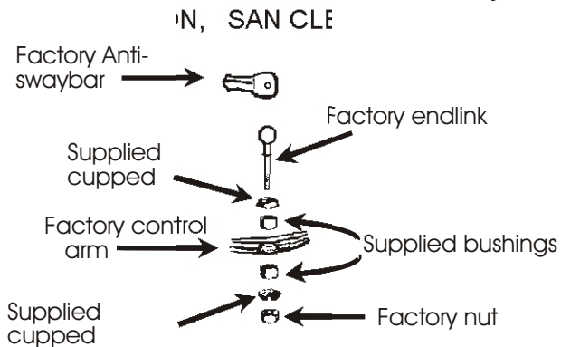
"Tie-rod style" endlink (uses only the parts shown above)
