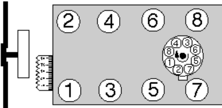
Figure 1- Chevrolet 265-400 c.i.d. V8 Firing Order 1-8-4-3-6-5-7-2 Turn distributor counter-clockwise to advance timing.
