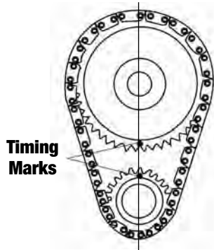
Figure 1 Timing Chain Sprocket Alignment Timing Marks
