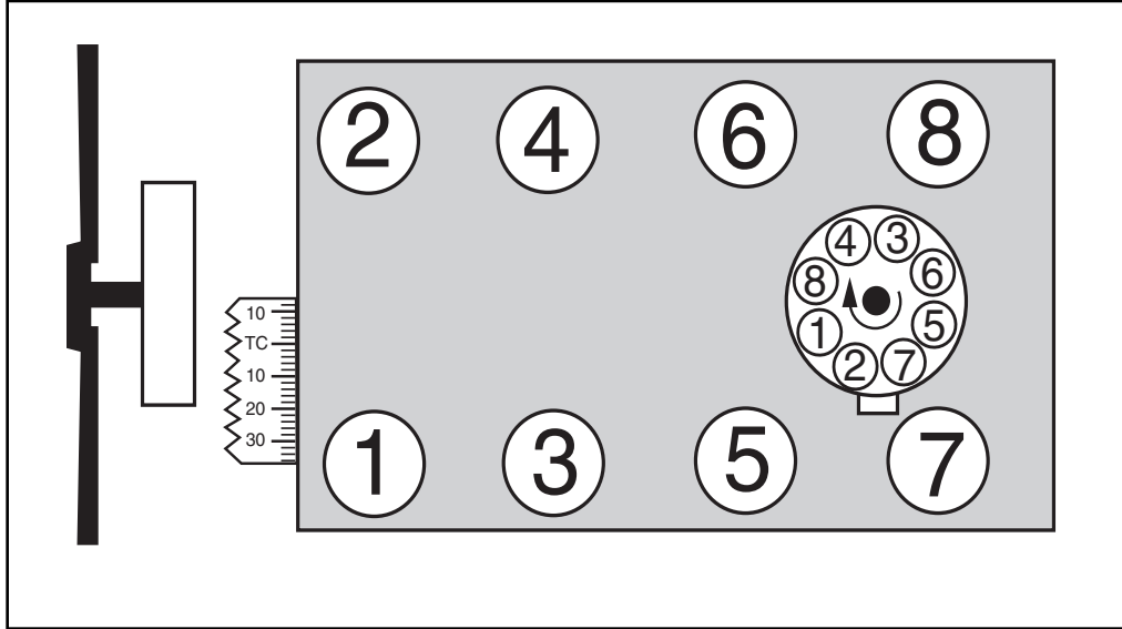
Figure 1- Chrysler 318-360 c.i.d. V8 Firing Order 1-8-4-3-6-5-7-2 Turn distributor counter-clockwise to advance timing.
