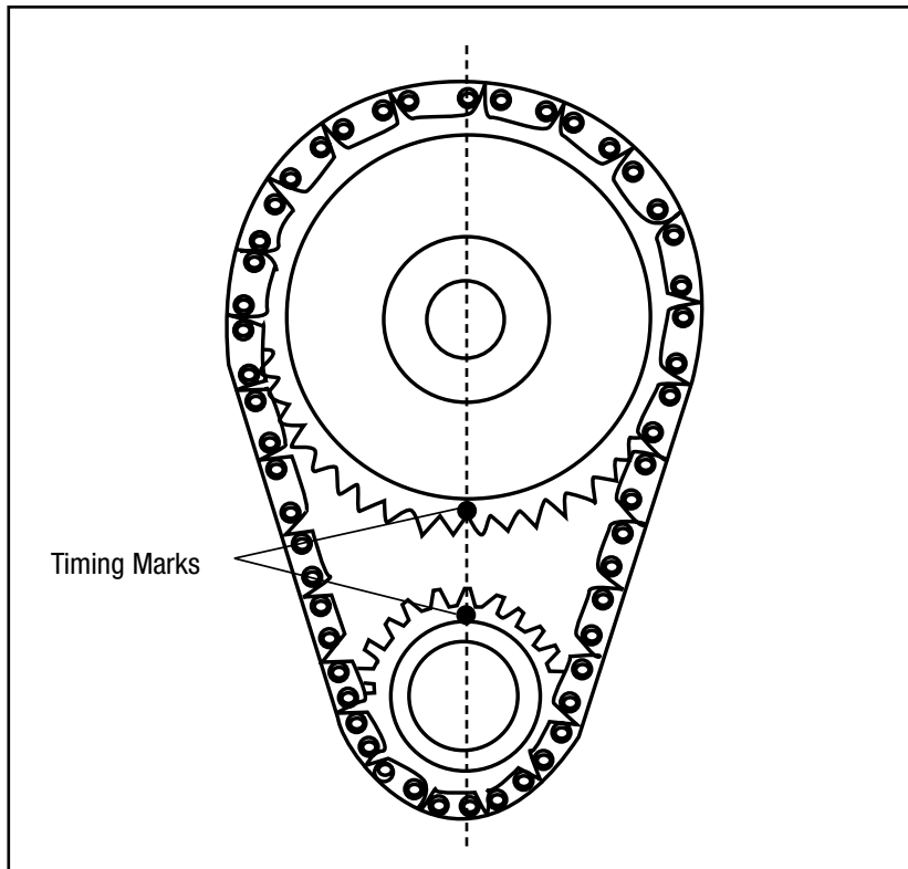
Figure 2- Timing Chain Sprocket Alignment
