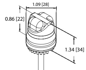
LED HEAD
