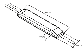
DRIVER MODULE
