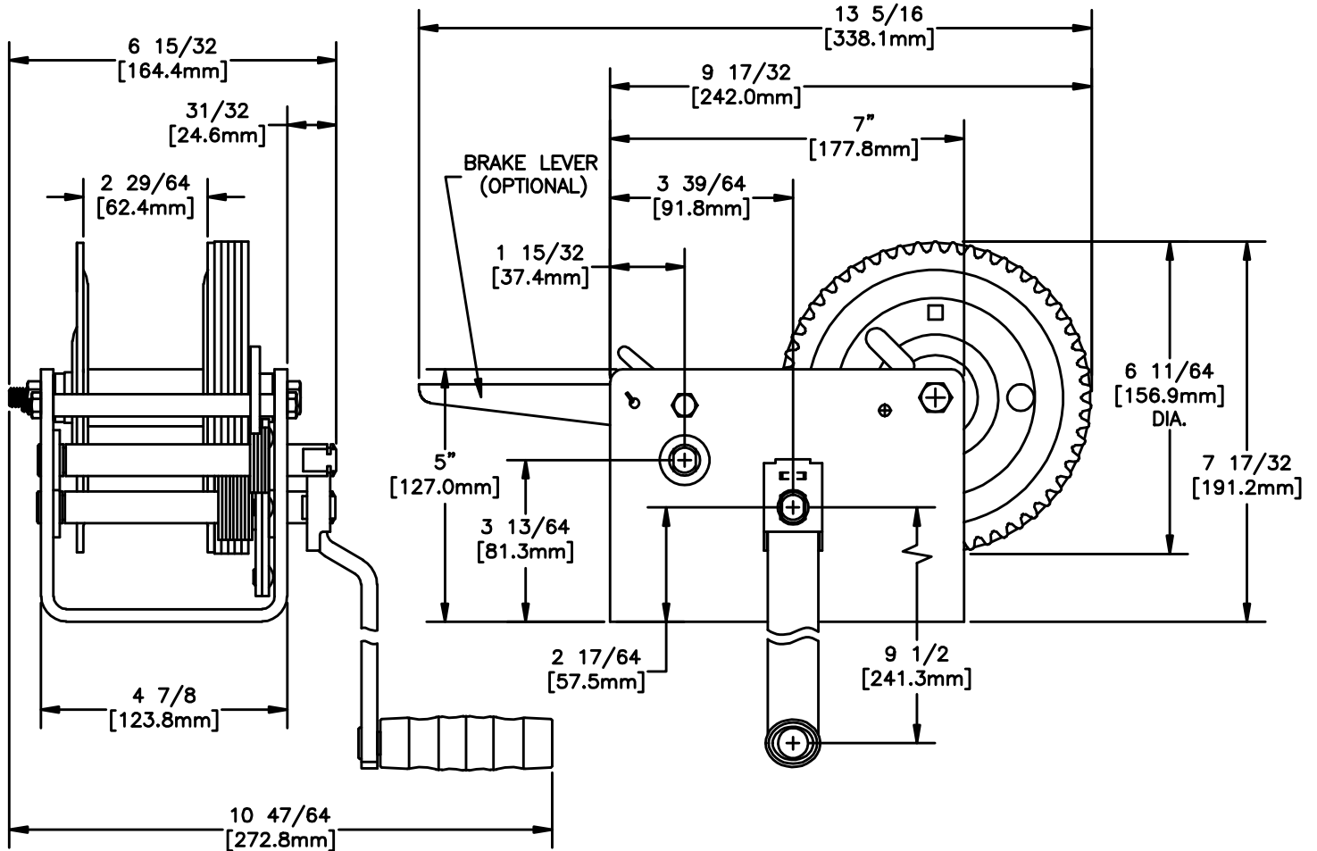
FRONT & SIDE VIEW
