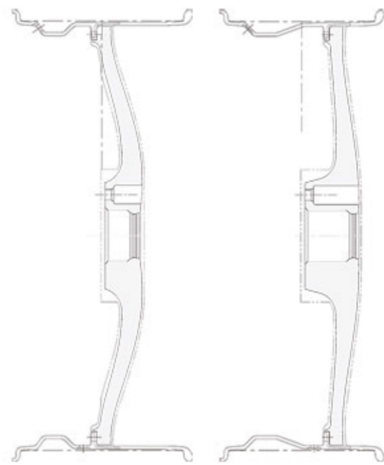
rear 5" lip front 3" lip
