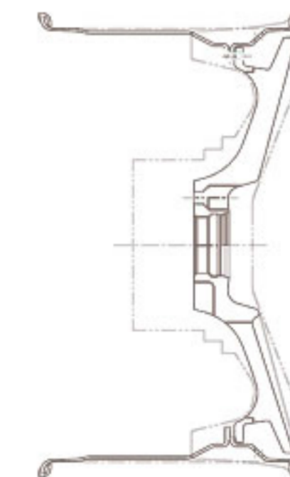
20x12 deep concave w/ floating spoke shown
