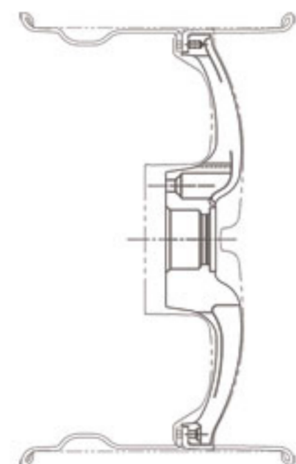
26" 3 pc. w/ 7" lip shown
