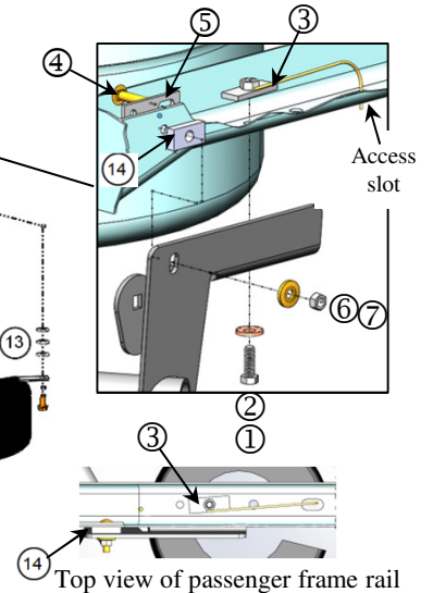
Top view of passenger frame rail
