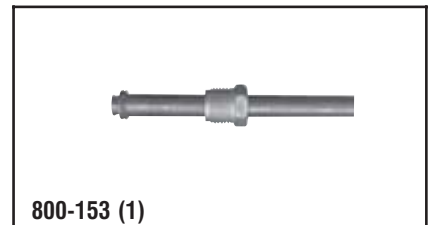
800-153 (1) Steel Fuel Line Repair 3/8" x 18" with 16mm compression fitting
