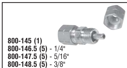
800-145 (1) 800-146.5 (5) - 1/4" 800-147.5 (5) - 5/16" 800-148.5 (5) - 3/8" Fuel Line Connector Assortment Nylon to Nylon 1/4", 5/16" & 3/8"
