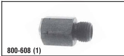
800-608 (1) Transmission Connector Ford 2000-82 w/ 5/16" Tube Connects transmission coolant line to radiator.
