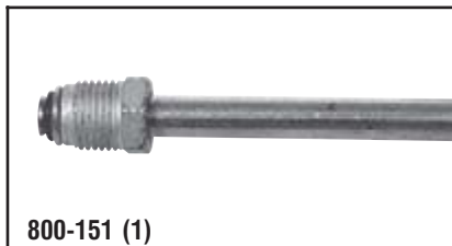
800-151 (1) Steel Fuel Line Repair 5/16" x 18" with 14mm compression fitting
