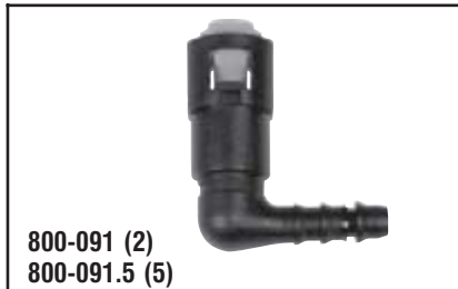
800-091 (2) 800-091.5 (5) Fuel Line Connectors 3/8" Steel to 5/16" (8mm) nylon elbow adapter
