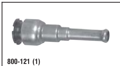
800-121 (1) Steel Fuel Line Repair 3/8" Body Connector for 3/8" hose and line
