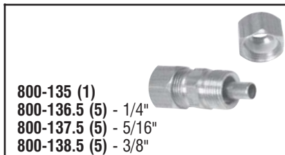
800-135 (1) 800-136.5 (5) - 1/4" 800-137.5 (5) - 5/16" 800-138.5 (5) - 3/8" Fuel Line Connector Assortment Nylon to Steel 1/4", 5/16" & 3/8"
