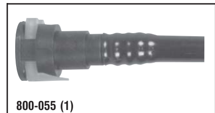
Nylon Fuel Line Repair Ford 3/8" Female x 5/16" tube
