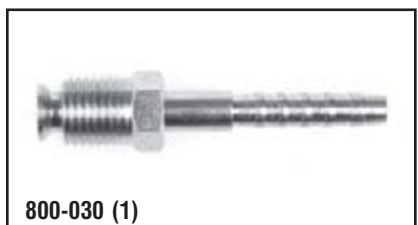
800-030 (1) Import Adapter M14 x 1.5 Flare to 5/16" Nylon Tube
