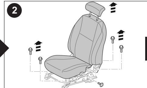
Remove seat and place on work bench for easy access.
