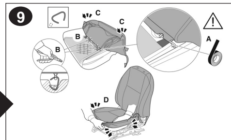
Replace cover - (clips, Velcro® and hog rings).
