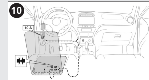
Layout wiring for connection before installing seat. Connect fuse tap to a fuse that is on with key in "Run" position to prevent battery drain when engine is off. Connect brown wire to solid metal ground point behind dash.
