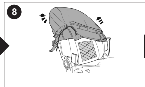
Install new pad, peel & stick adhesive. Note: Be sure to route wiring to bottom of seat back, away from center of the seat.
