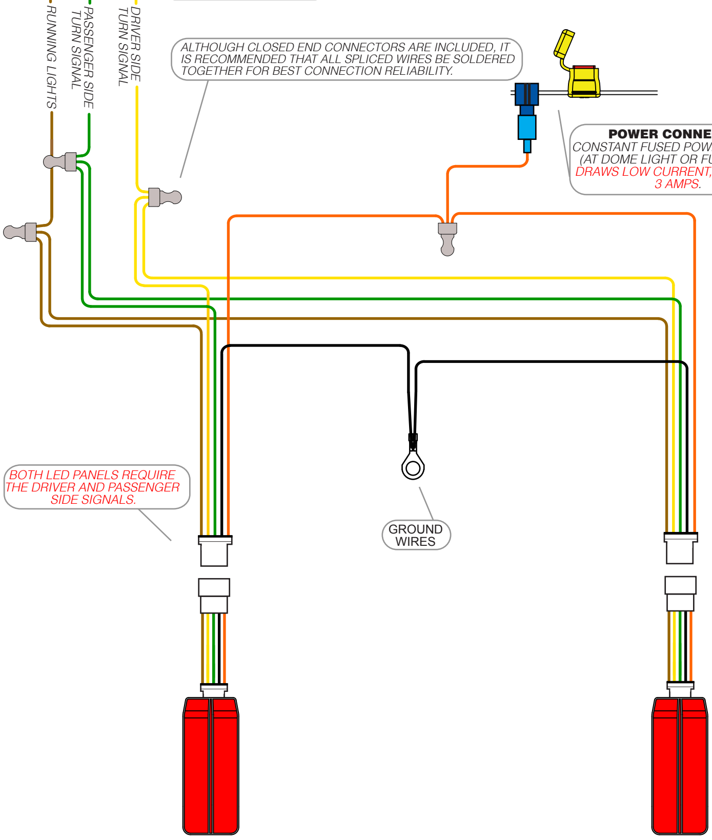
DRIVER SIDE LED PANEL
