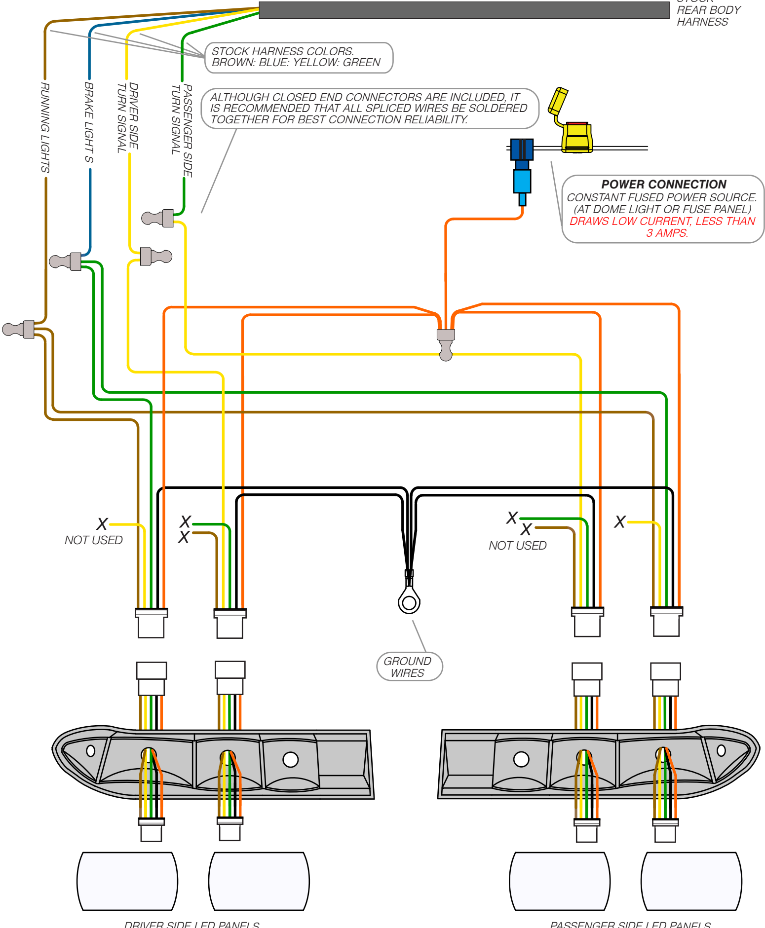
DRIVER SIDE LED PANELS
