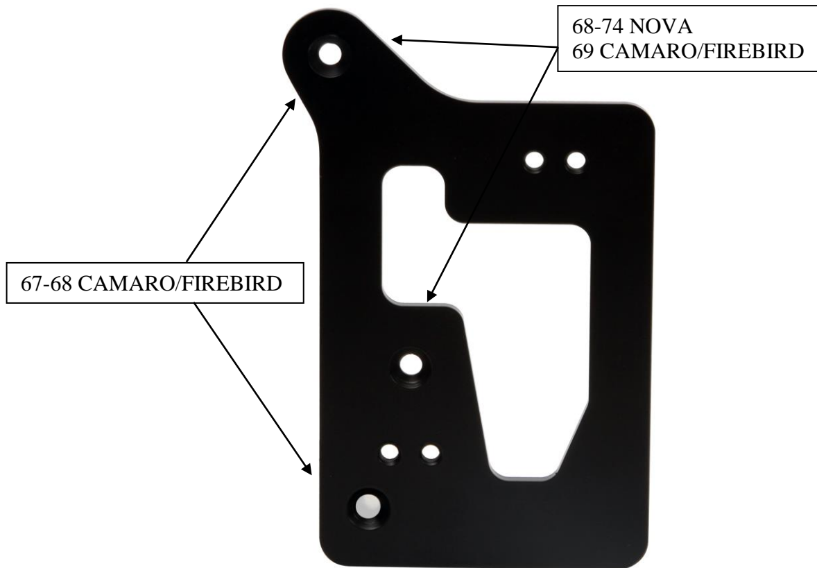
Figure 1 - C6 Throttle Pedal Bracket
