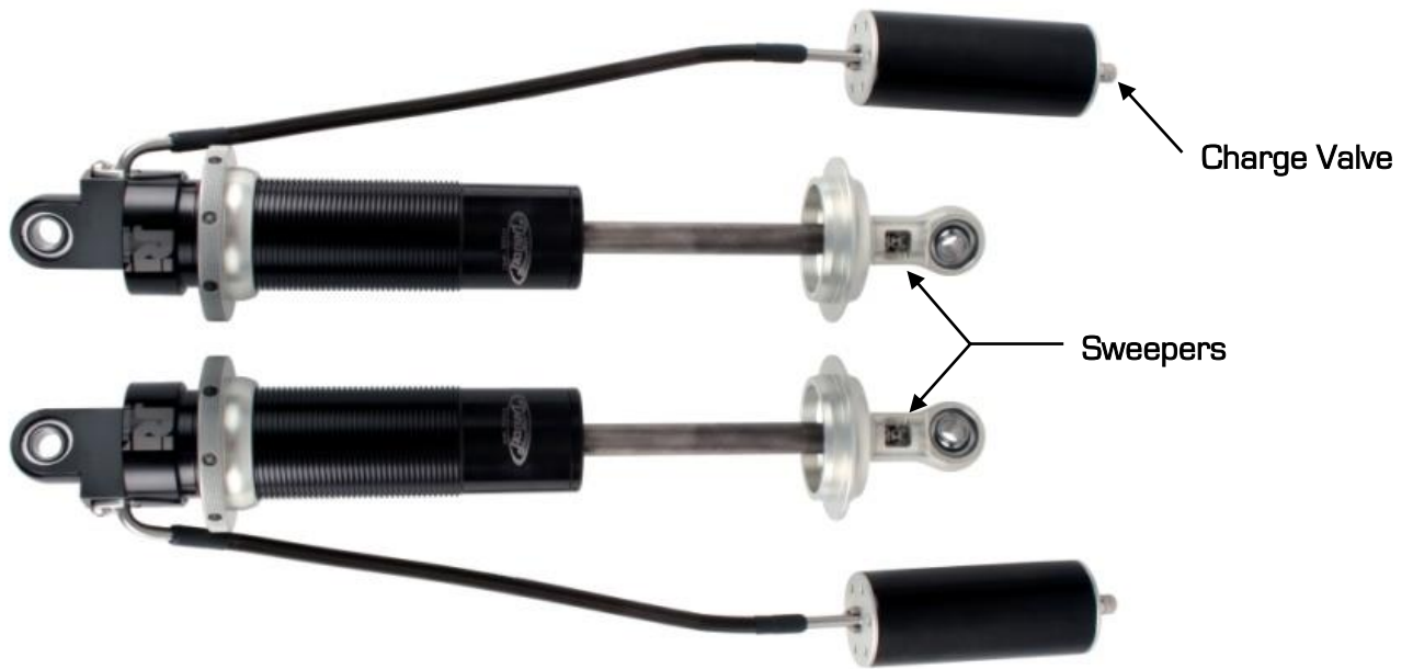
Figure 6 - Detroit Speed Double Adjustable Shock w/Remote Canister
