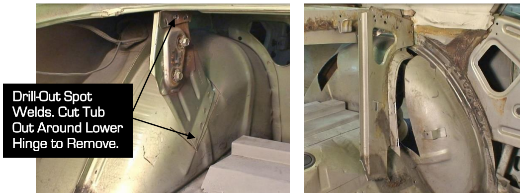
Figure 4 - Remove Seat Support & Decklid Hinge (Coupe)
