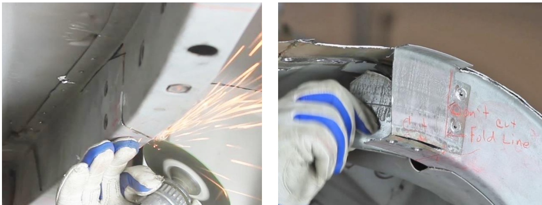
Figure 16 - Remove Frame Rail Section
