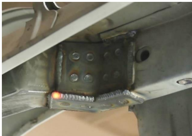
Figure 25 - Weld Bottom Frame Rail Doubler Plate
