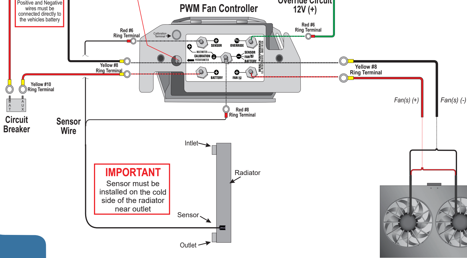
Dual Electric Fan Setup
