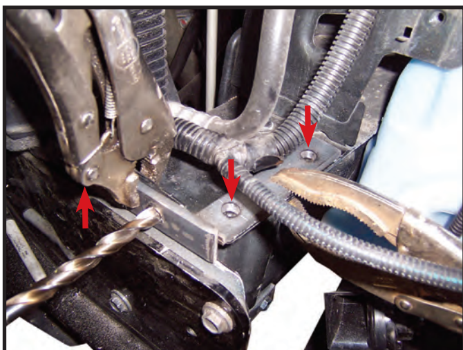
16. Clamp upper bracket to frame as shown. Make sure bracket is flush with the pinch weld on the side. Drill four 13/32" holes using bracket as a template. Repeat on other side.
