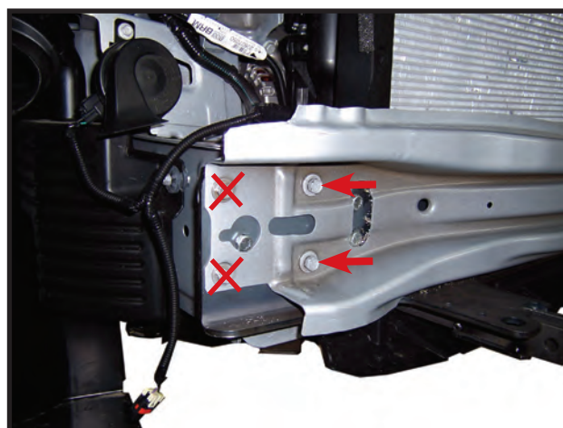
19. Remove factory bumper bolts and reinstall bumper using factory bolts in inside holes of bumper. NOTE: Use blue LOCTITE on all bolts and tighten all bolts according to chart on front page.
