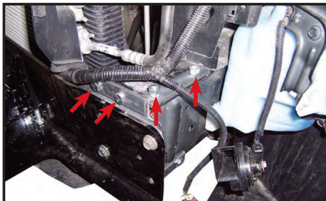
17. Place 3/8 x 1" bolts thru drilled holes and place 3/8" lock washer and 3/8" nut behind frame. NOTE: Use blue LOCTITE on all bolts and tighten all bolts according to chart on front page. Reinstall bolt holding horn on both sides.
