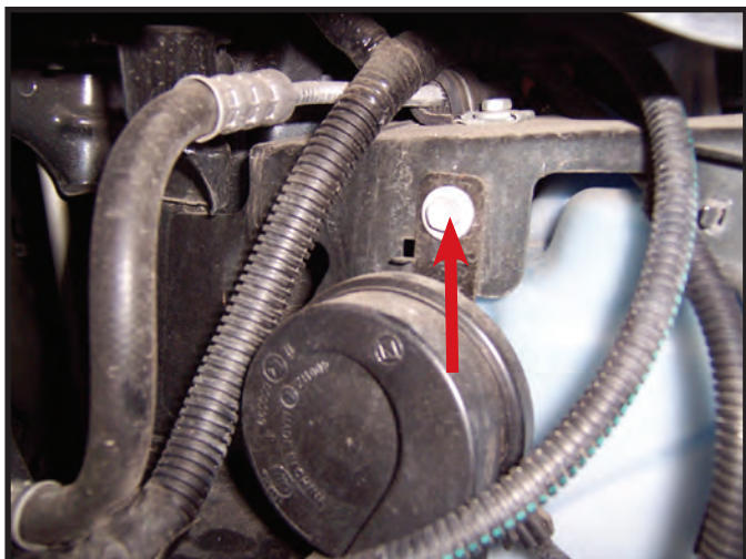
14. Remove one bolt on each side from horn and let hang.
