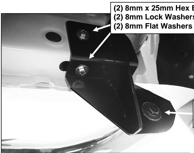
(Fig 12) Passenger/right rear Bracket installation
