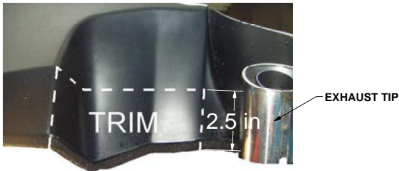
TRIM DIAGRAM FOR 2011 MODELS (PASSENGER SIDE SHOWN - TRIM BOTH SIDES)
