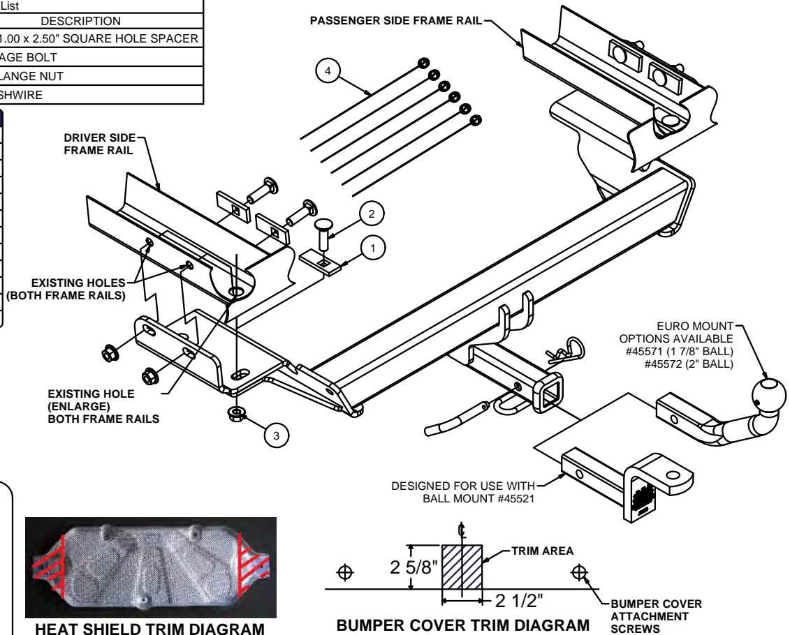
HEAT SHIELD TRIM DIAGRAM
