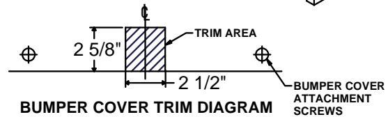
BUMPER COVER TRIM DIAGRAM
