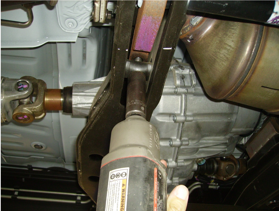
Figure 1: remove torsion bar adjusting bolt
