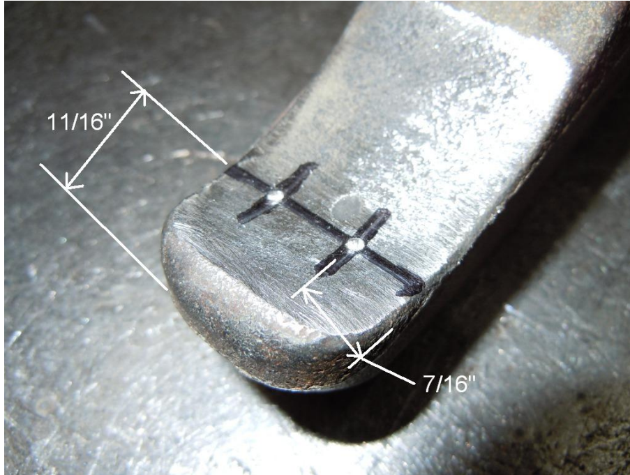
Figure 17: Center punch 2 spots, 11/16" from the end and 7/16" from each side.
