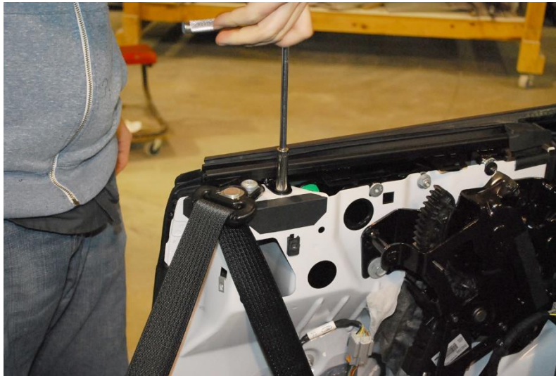
14. Remove 15mm convertible top fastener. Set aside to reinstall.
