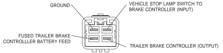
Wiring Adapter Housing (containing Male Terminals) - Pin Side (Mating Side)
