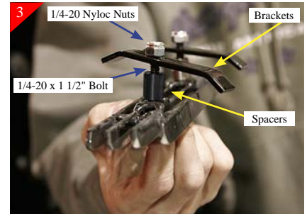
Start by placing supplied 1/4-20 x 1 1/2" bolt thru mounting tab in billet grille . Then place the supplied spacers on bolts, followed by the brackets & 1/4-20 nyloc nuts. Repeat process for all remaining billet grilles.
