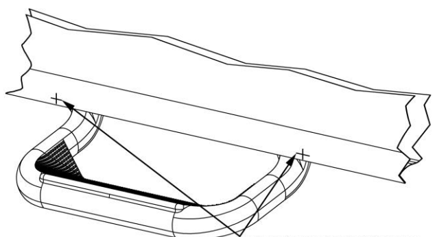
MARKED HORIZONTAL LINES 1/2" UP FROM BOTTOM OF PINCH WELD
