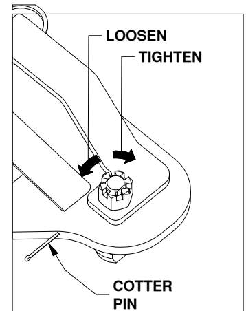
FIGURE C4: View of base leg.
