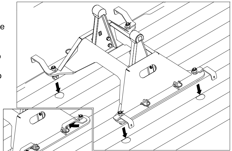
FIGURE C1: View of unlatched base
