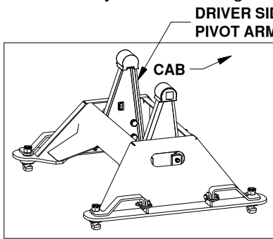
FIGURE B3: View of base.
