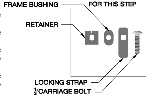
ROTATE THE LOCKING STRAP CLOCKWISE UNTIL IT HITS THE BOTTOM OF THE TRUCK FRAME
