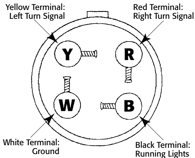
Magnetic Towing Light Connector Schematic
