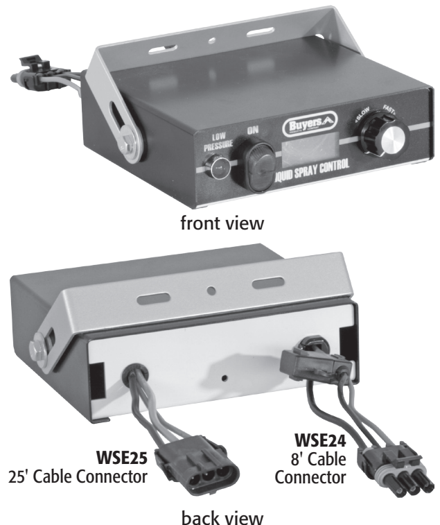
Fig. 7 WSE1 Cab Controller
