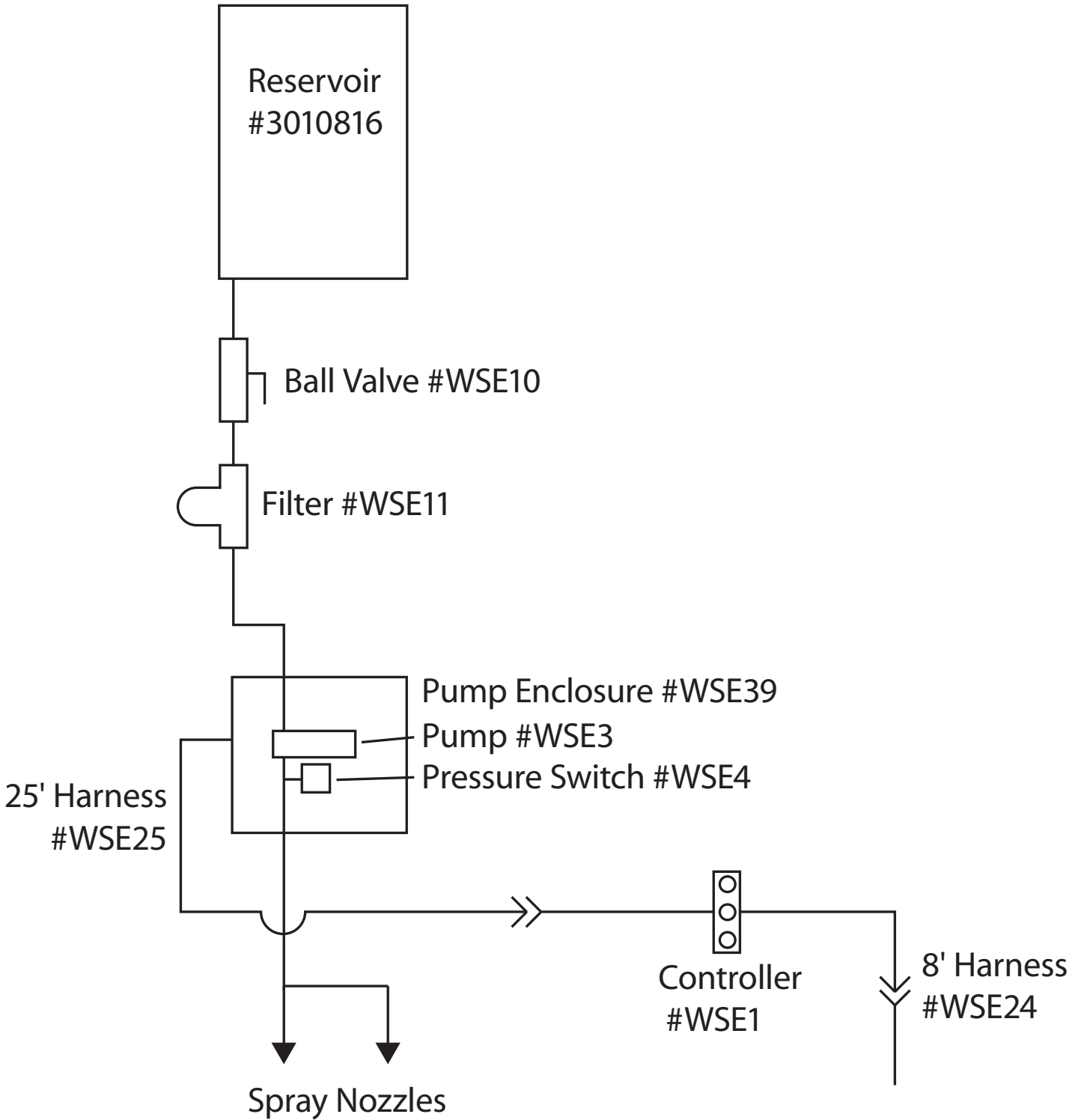
Fig. 8 Plumbing Dia.
