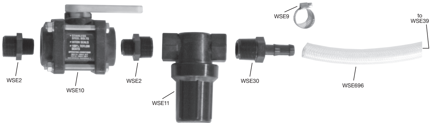
Fig. 10 Filter/Valve Assembly
