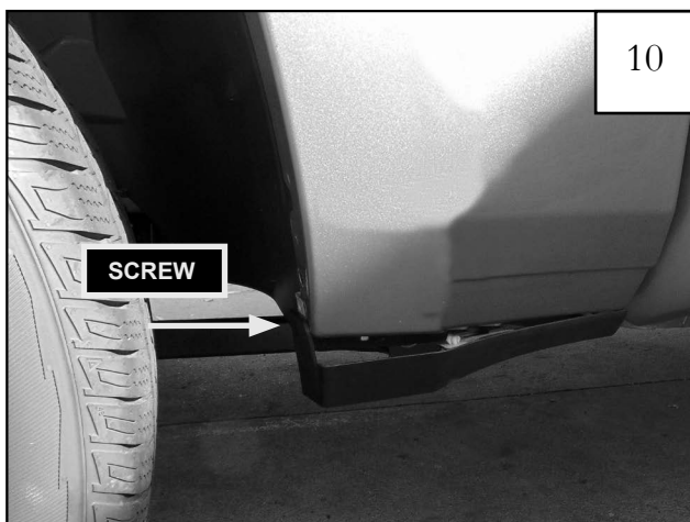
Remove and keep (1) factory installed screw, and remove mud flap from vehicle. This factory screw will be used to install the rear fender flare.
