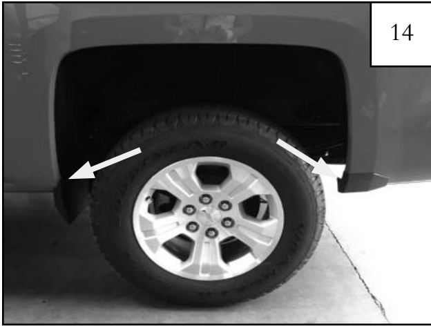
Using a T-15 Torx bit socket wrench, remove factory installed screws using. Discard screws.
