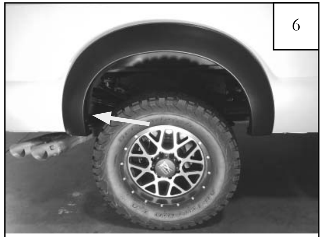
Install a 5/16" Phillips Truss Screw (SW1-0050) into the "S" clip over the rear most hole.
