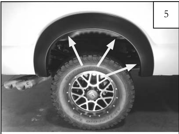
Position the flare on the fender and install a 5/8" Phillips Truss Screw (SW1-0058) into each of the three "U" clips installed in the previous step.
