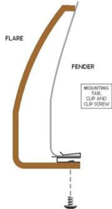
Illustration #3 Cross Section of Flare and Fender With Tab, Clip (Front & Rear) and Screw
