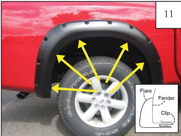
Passenger Side Flare: Install five Clips (CL1-0005) over fender lip, lining up the hole in Clips with the holes in flare. Start Screws (SW1-0050) in each Clip. Do not fully tighten screws.
