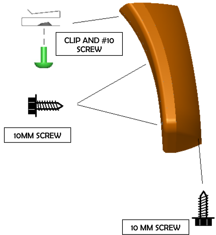
Illustration #5 Access Door Flare Without Mud Flaps
