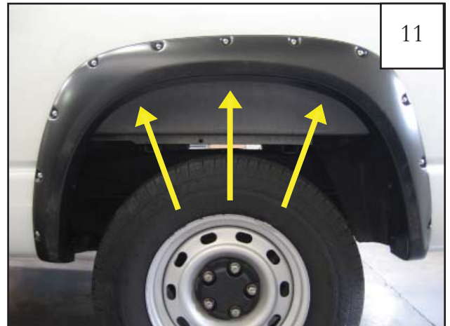
Hold flare in place and mark three locations with a grease pencil using the holes in the flare as a guide. See step 12 & 13.
