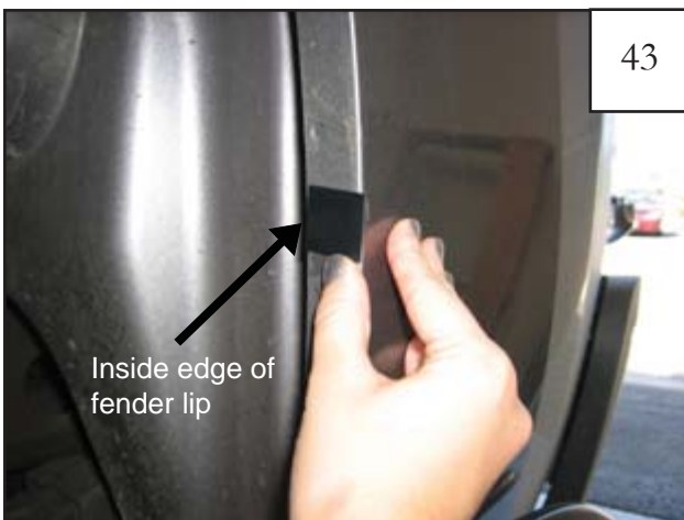
Center a supplied Tab (MT1-0002) over the marks made in step 41, aligning edge of tab with inside edge of fender lip (tab may extend over outside of fender).
